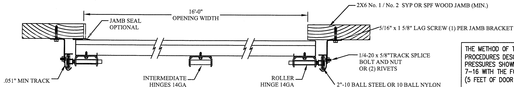
2" BRACKET MOUNT TO WOOD JAMB DETAIL
