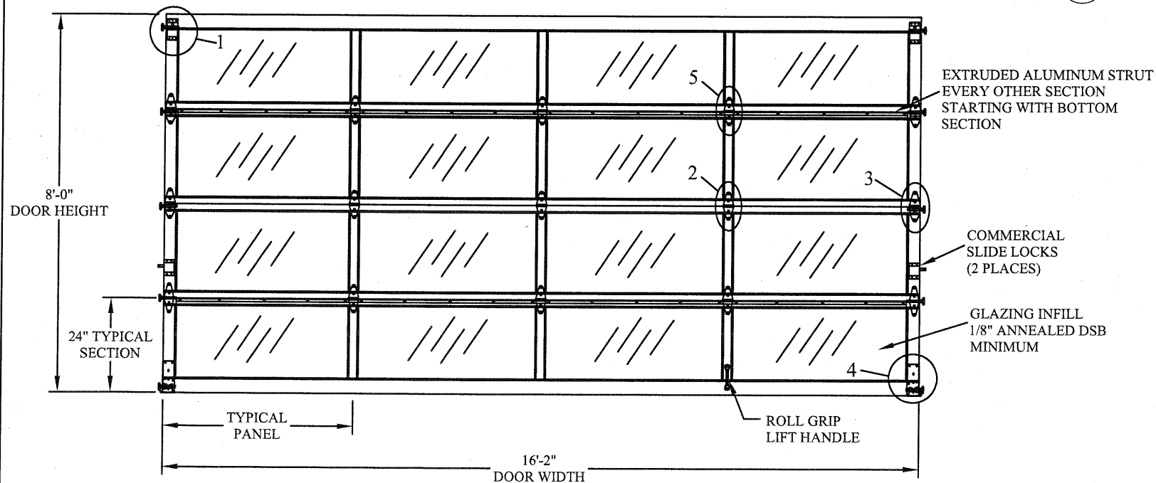
DOOR INTERIOR ELEVATION
