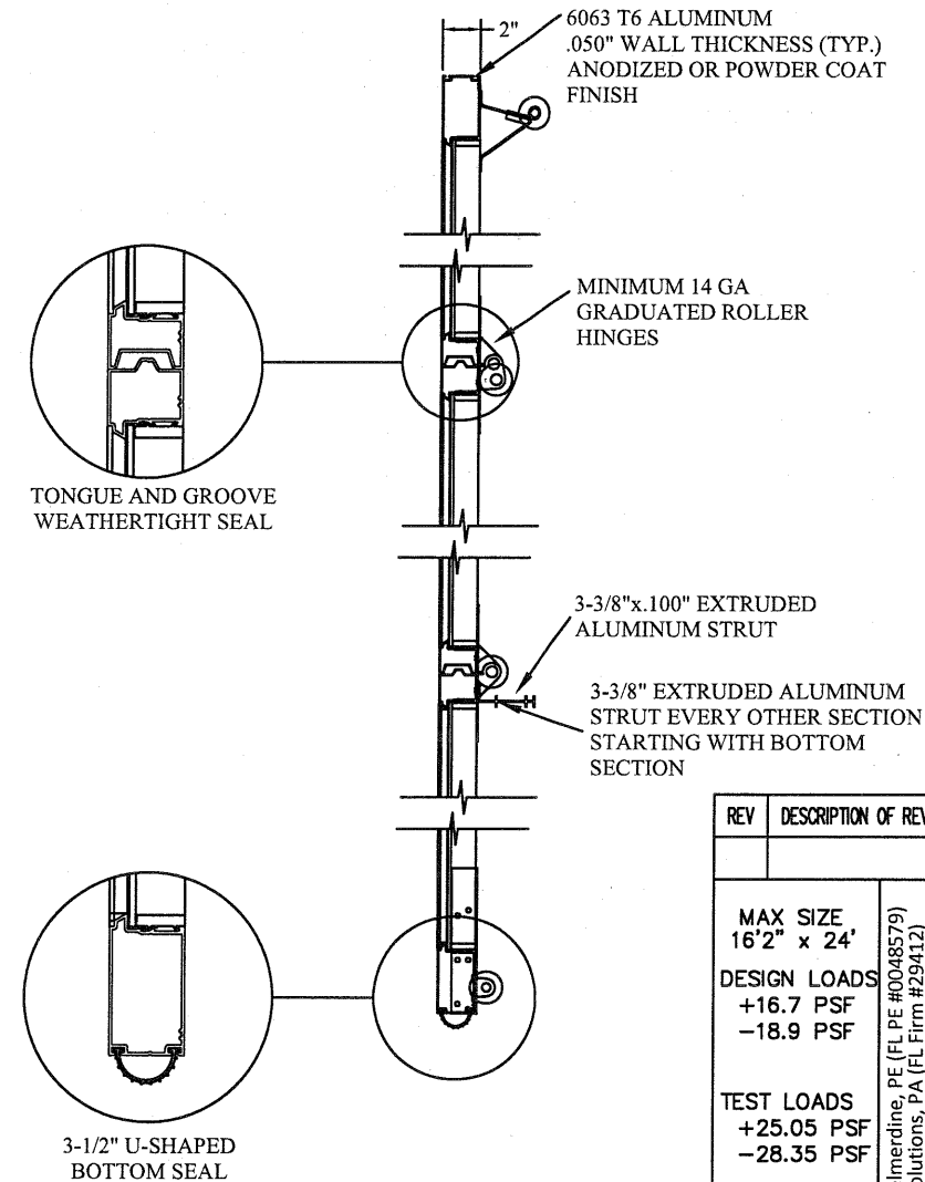
ALUMINUM SECTION PROFILE
